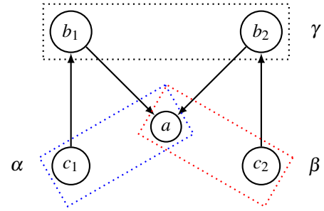
Figure 3: There is no single agent defending argument a
